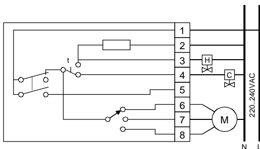
RTC3000B
