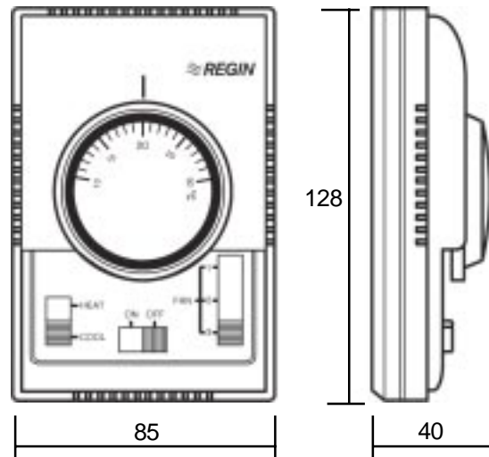
RTC3000A shown
