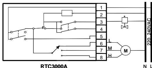
RTC3000A
